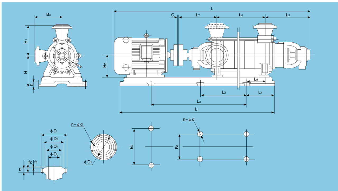
D、DG、DF、DY、DM型泵外形安装图(本身底座) (With Pump Base)
